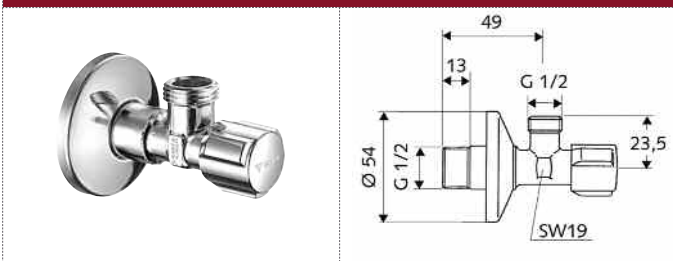
97 058 00 00 SCHELL llave Comfort
